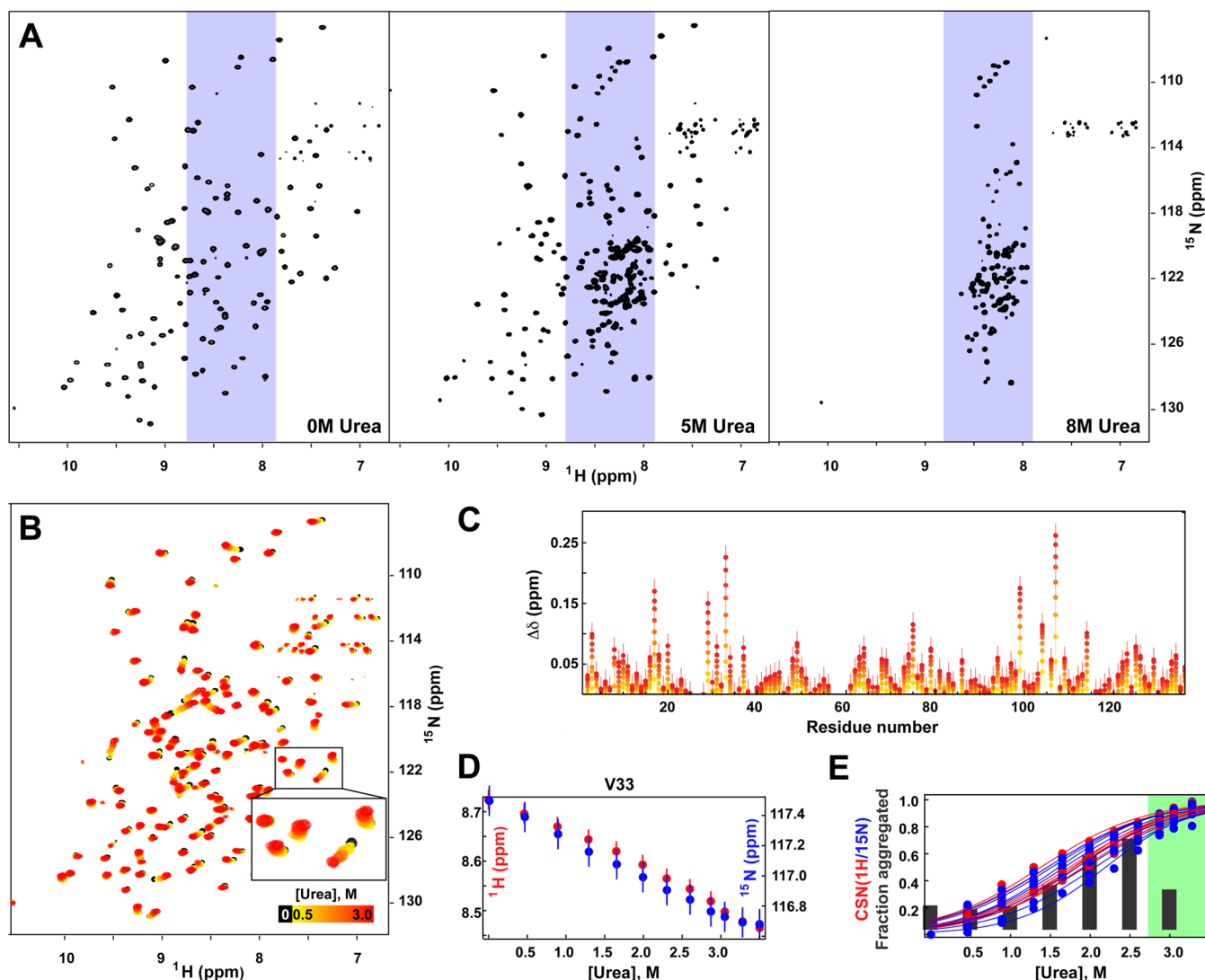
Figure 3. Urea results in two transitions in CRABP1 WT*: near-native transition at low urea concentrations and protein unfolding at high urea concentrations. (A) ^1\text{H} , ^{15}\text{N} HSQC NMR spectra of CRABP1 WT* in the absence (left) and presence of 5 (middle) and 8 M (right) urea. (B) ^1\text{H} , ^{15}\text{N} HSQC NMR spectra of CRABP1 WT* in the absence (black) and presence of 0.5–3.1 M urea (colored from yellow to red as the urea concentration increases). (C) Amide proton chemical-shift (CS) perturbations in the presence of 0.5–3.1 M urea, \text{mod}[\Delta\delta(\text{urea}) - \Delta\delta(\text{no urea})] , colored as in panel B. (D) CS dependences of amide ^1\text{H} (red) and ^{15}\text{N} (blue) as a function of urea concentration for a representative residue (V33); see also Figure S1. (E) Aggregation propensity of CRABP1 WT* (gray bars, same as red bars in Figure 2) and fractions of the aggregation-prone near-native conformation (calculated as normalized CS dependences of amide ^1\text{H} (red) and ^{15}\text{N} (blue) [\Delta\delta(\text{urea}) - \Delta\delta(\text{no urea})]/[\Delta\delta(3.5 \text{ M urea}) - \Delta\delta(\text{no urea})] ; individual data points correspond to particular highly affected residues) as a function of urea concentration; see also Figure S1. A green region indicates the higher urea concentrations that result in aggregate instability.
