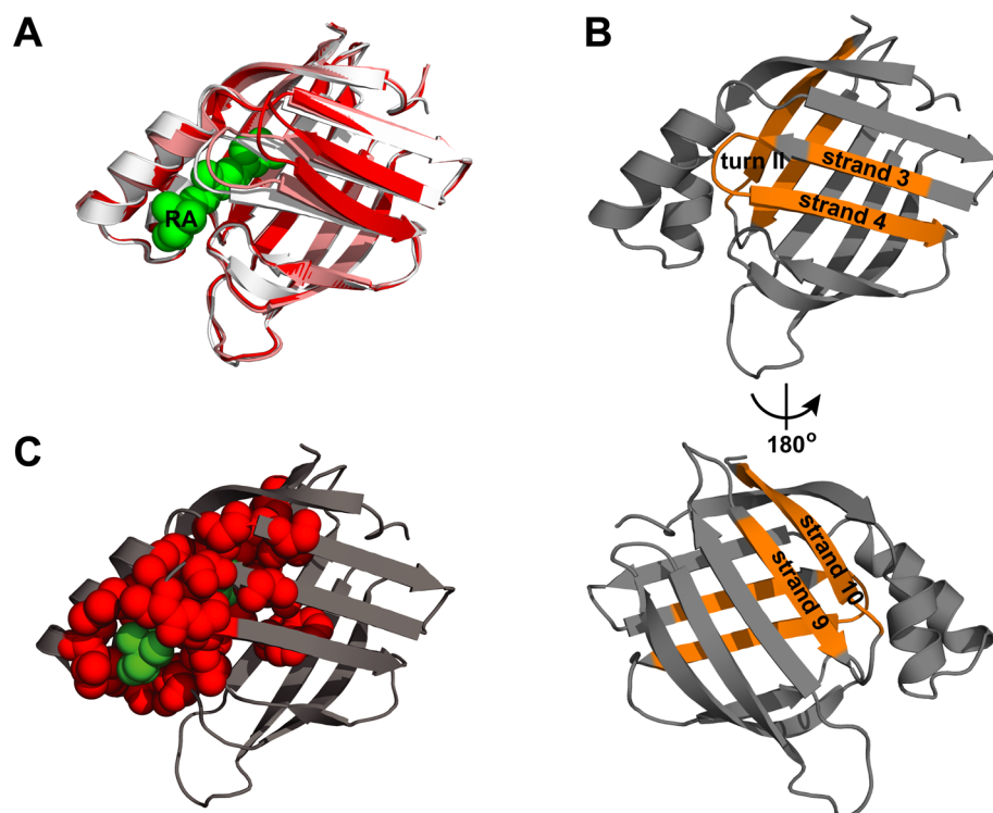
Figure 1. Structural features of folded CRABP1 and its amorphous aggregates. (A) Overlay of the X-ray structures of holo-CRABP1 (PDB ID 1CBR, chain A, white) and apo-CRABP1 (PDB ID 1CBI, chain A, red, and chain B, pink). The RA molecule is shown in green. (B) Two aggregation cores of CRABP1 (strand 3-turn II-strand 4 and strand 9 and 10, orange) mapped onto holo-CRABP1 (PDB ID 1CBR, chain A) (as reported by Budyak et al. 25 ). (C) Conserved ligand-binding residues (red spheres) in the iLBP family (as defined by Marcelino et al. 49 ) mapped on the X-ray structures of holo-CRABP1 (PDB ID 1CBR, chain A). The RA molecule is shown in green.
