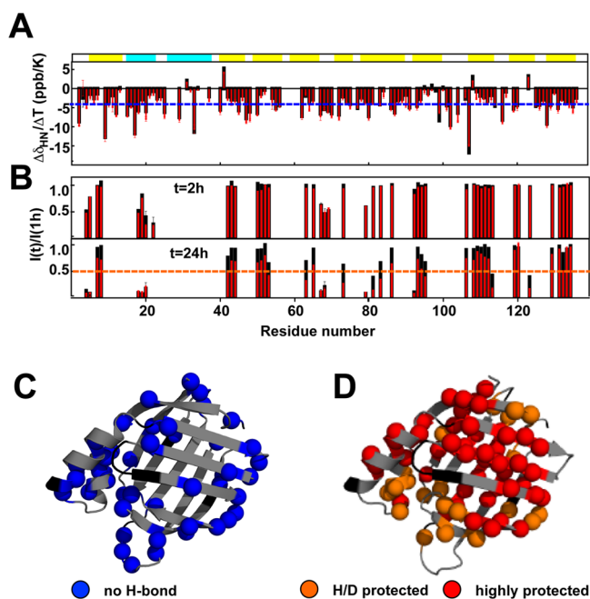
Figure 4. Native and aggregation-prone CRABP1 conformations share the same structural features. (A) Amide temperature coefficients ( \Delta\delta_{HN}/\Delta T ) of CRABP1 WT* in the absence (black) and presence (red) of 1.5 M urea. (B) Deuterium incorporation after 2 and 24 h of H/D exchange in the presence (red) and absence (black) of 1 M urea, I(t)/I(1h) , where I(t) is the peak intensity after 2 or 24 h of exchange and I(1h) is the intensity for the corresponding peak after 1 h of exchange. (C) CRABP1 WT* residues involved in hydrogen bonding determined from the amide temperature coefficients from panel A (i.e., \Delta\delta_{HN}/\Delta T > -4.5 ppb/K) mapped on the X-ray structure of CRABP1 (PDB ID 1CBP, chain A). The same residues were identified in the absence and presence of 1.5 M urea (see panel A). (D) Mapping of CRABP1 WT* residues that are highly (red, I(24)/I(1) > 0.5 ) and moderately (yellow, I(24)/I(1) < 0.5 and I(24)/I(1) > 0.2 ) protected from the solvent, as determined from H/D-exchange measurements. The same groups of residues were identified in the absence and presence of 1 M urea (see panel B).
