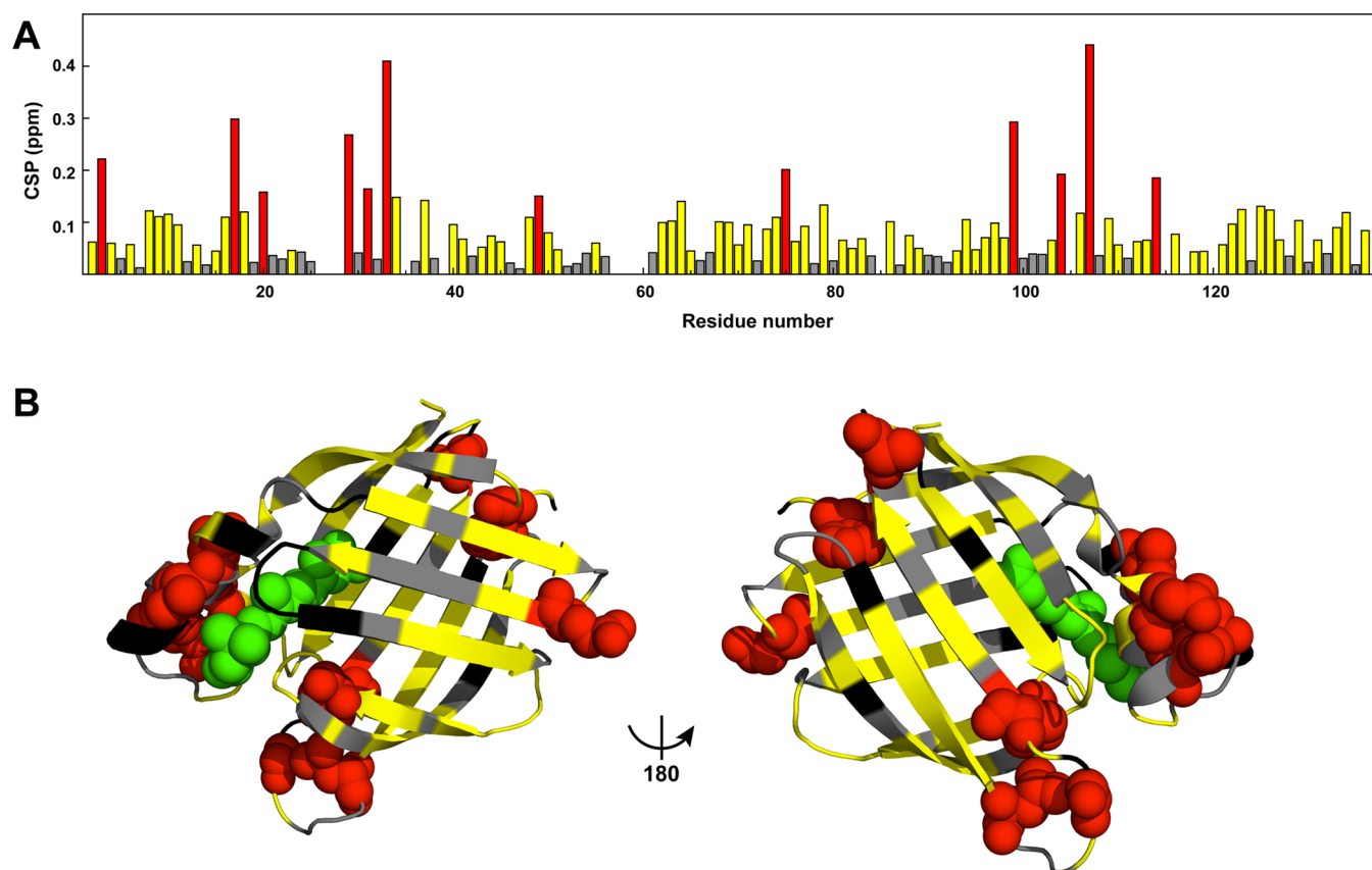
Figure 5. Aggregation-prone conformation of CRABP1 affects the ligand-entry portal. (A) Chemical-shift perturbations (CSPs) as a function of residual number. CSPs were determined as [\Delta\delta_H^2 + (0.154\Delta\delta_N)^2]^{1/2} , where \Delta\delta_H and \Delta\delta_N are amide proton and nitrogen differences in the chemical shifts between CRABP1 WT* in the absence and presence of 3.5 M urea. Residues with large CSPs (>0.14 ppm) and significant CSPs (>0.035 ppm) are colored red and yellow, respectively; the rest are shown as gray. (B) Mapping of CSPs from panel A into the X-ray structure of CRABP1 (PDB ID 1C8R, chain A). Residues with significant and large CSPs are colored as in panel A.
