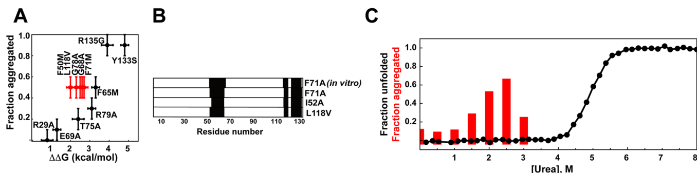
Figure 2. Origin of aggregation propensity in CRABP1 is more complex than a simple increased fraction of the unfolded protein. (A) Aggregation propensity (a fraction of insoluble protein) of different CRABP1 WT* mutants as a function of protein destabilization upon single point mutations (see also Table S1). (B) Aggregation cores of different CRABP1 WT* aggregation-prone variants (F71A, I52A, and L118V) obtained from E. coli inclusion bodies using DMSO-quenched H/D-exchange experiments and previously reported aggregation cores obtained in vitro using the F71A variant of CRABP1 WT*. 25 (C) Aggregation propensity of CRABP1 WT* (red, monitored as a fraction of insoluble protein) and fraction of unfolded CRABP1 WT* (black, monitored by intrinsic tryptophan fluorescence spectroscopy) as a function of the urea concentration.
