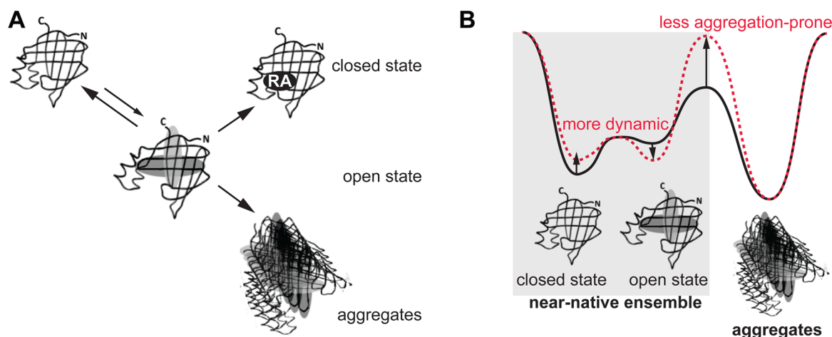
Figure 7. Interplay between conformational flexibility and aggregation in the iLBP family. (A) Schematic representation of transitions from the near-native CRABP1 ensemble. The population of the open, aggregation-prone conformation is required for ligand binding but also results in aggregation. (B) Energy landscape of iLBPs under native conditions comprises a delicate balance between protein conformational flexibility and aggregation. The iLBP near-native conformational ensemble comprises at least two conformations: a closed, ‘secure’ conformation and an open, ‘at-risk’ conformation that is essential for ligand binding but may promote aggregation. The fine-tuning of thermodynamic and kinetic features of the landscape prevents different iLBP members from aggregation and allows them to perform their specific function. Rigid iLBPs such as CRABP1 (black) minimize the amount of time that proteins spend exposing the hydrophobic regions to be efficient enough for ligand binding but not sufficient for aggregation. The Lb-FABP/LFABP/iLBP subfamily members (red) spend significant amount of time in the open conformation, allowing binding to larger ligands. To avoid aggregation, regions exposed in the open conformation are less hydrophobic.
